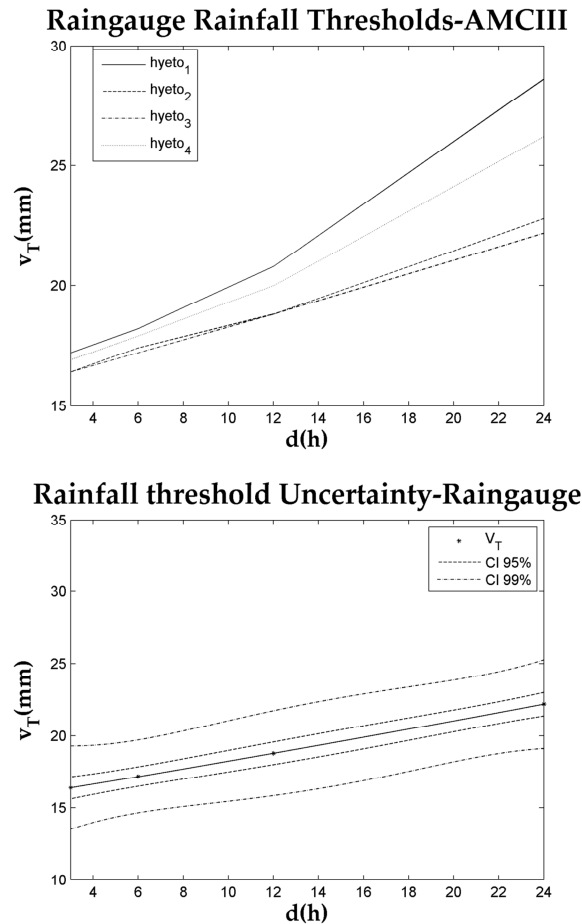
Fig. 9. Threshold values evaluated by a hydrological model calibrated with raingauge data for AMCIII soil conditions (upper panel) and uncertainty associated with hyeto_1 threshold for the Mignone River basin (lower panel).
