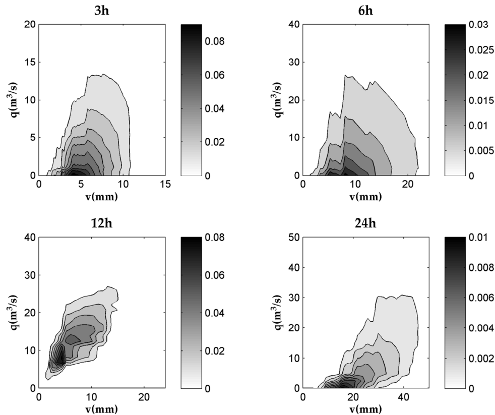
Fig. 3. Joint probabilities distributions for rainfall depth-cumulated rainfall (3, 6, 12, 24 h), for soil AMCIII condition.
