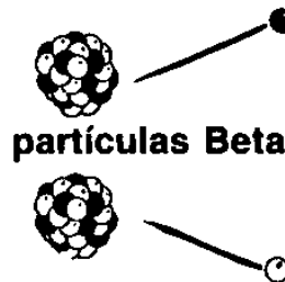
FIG. 3. Atomos inestables.
