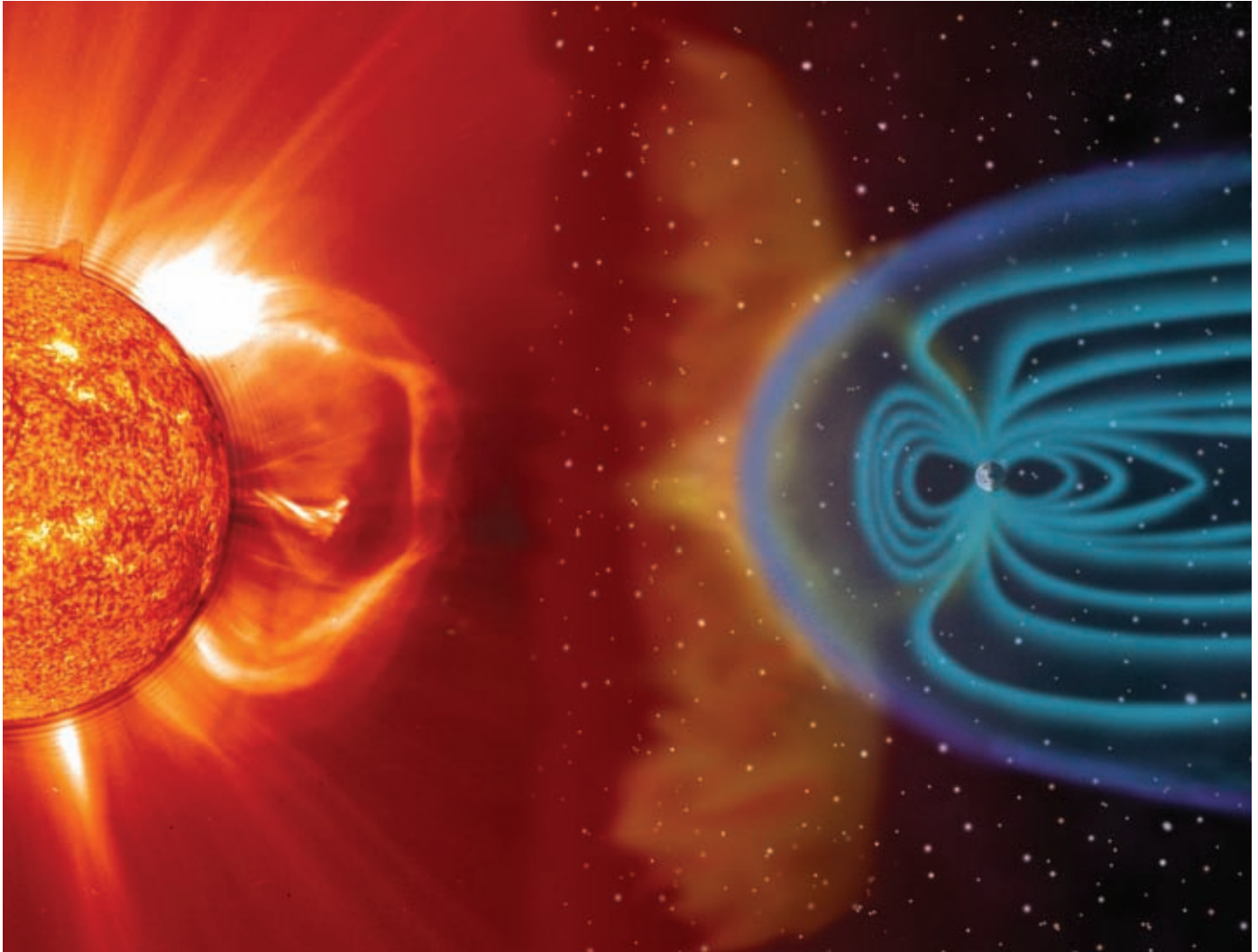
Figure 2: The space weather environment © NASA
